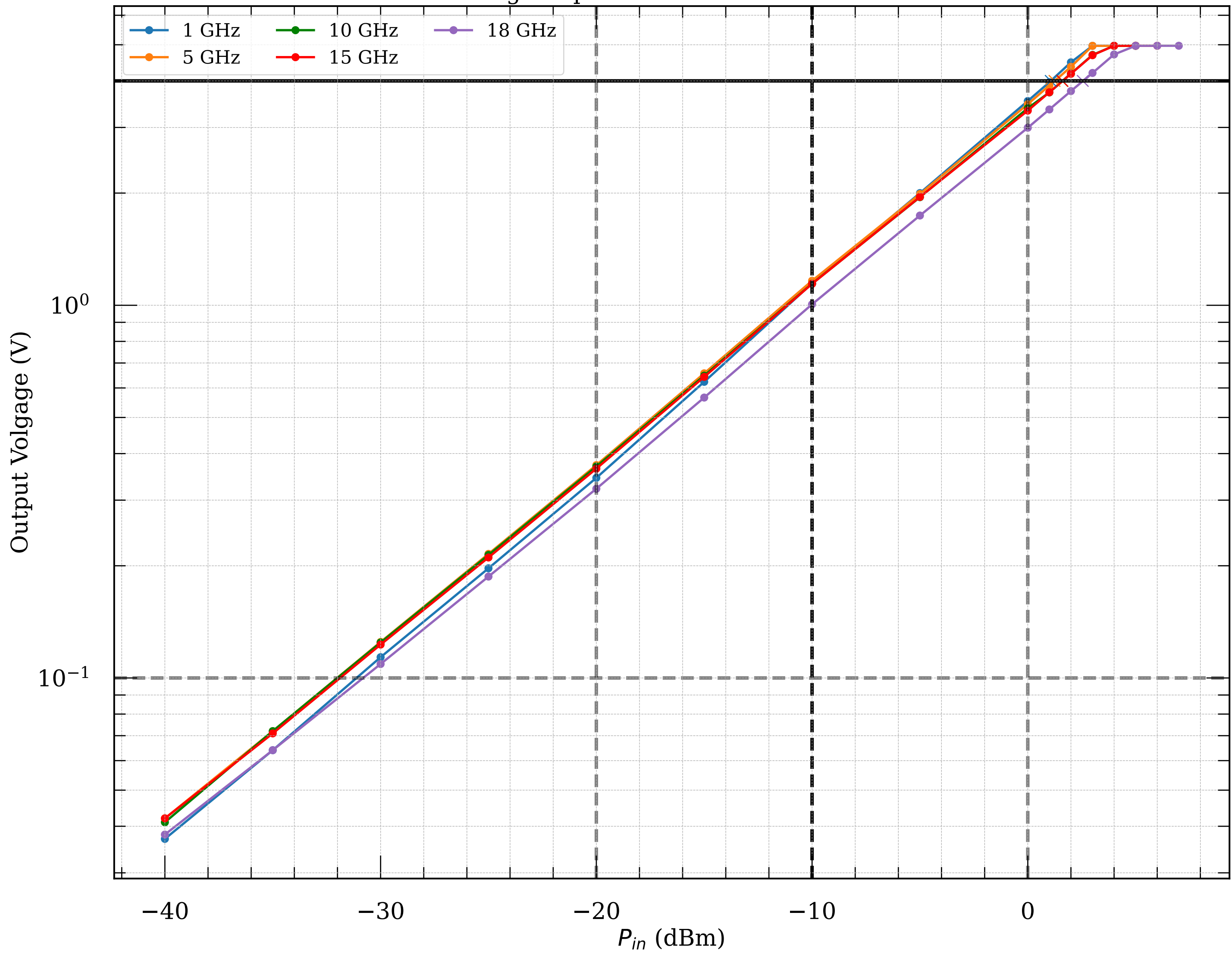
Measured voltage-to-power curve of detector module024v2
